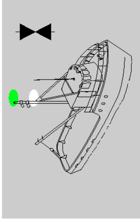
Vessel engaged in trawling—not making way; vessel less than 50 meters in length. Same for International.
