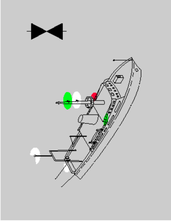
Vessel engaged in trawling—making way. Same for International.
